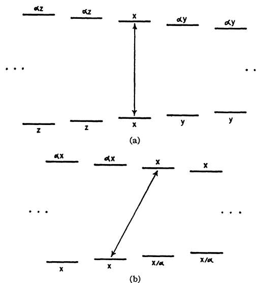
FIG. 2. (a) The populations of the hyperfine levels which result from the saturation of an allowed transition when the relaxation rates W_0(m) and W_2(m) are comparable. The values of x , y , and z are calculated in Sec. II. (b) The populations produced by saturation of a forbidden transition when W_1(m) is fast and \Phi_2 = 0 .
