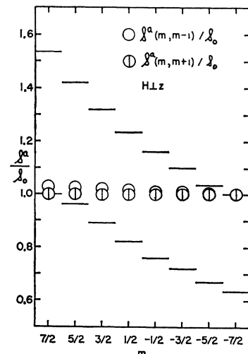
FIG. 6. The measured signals from T_1(m) when T_1(m+1) and T_1(m-1) are saturated, for H \perp z . The histograms are drawn according to the theory of Sec. II, with R_m = \infty .
