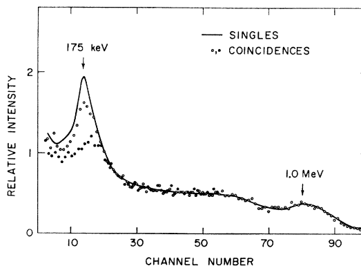
FIG. 8. Gamma spectra of Sc^{48} : (a) singles spectrum —, (b) spectrum in coincidence with 316 \pm 13 keV electrons —○, and (c) spectrum in coincidence with 534 \pm 21 keV electrons —●.
