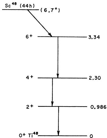
FIG. 1. Decay scheme of Sc 48 .
