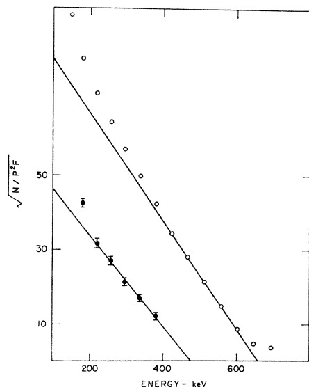
FIG. 6. Kurie plot of beta spectrum of Sc^{48} .
