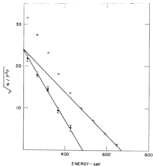
FIG. 7. Kurie plot of beta spectrum of Sc^{48} in coincidence with 175-keV gammas.
