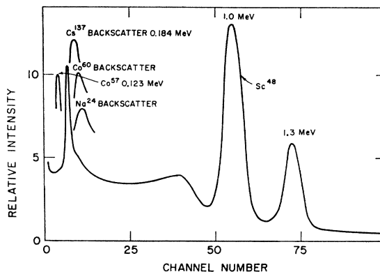
FIG. 2. Gamma spectrum of Sc 48 .
