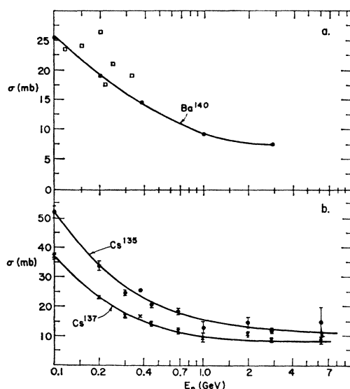
FIG. 3. Excitation functions for cumulative formation of neutron-excess nuclides. (a) Ba 140 . The open squares are data from reference 22, normalized to the Al( p ,3 p n ) cross sections used in the present paper. (b) Cs 135 and Cs 137 .
