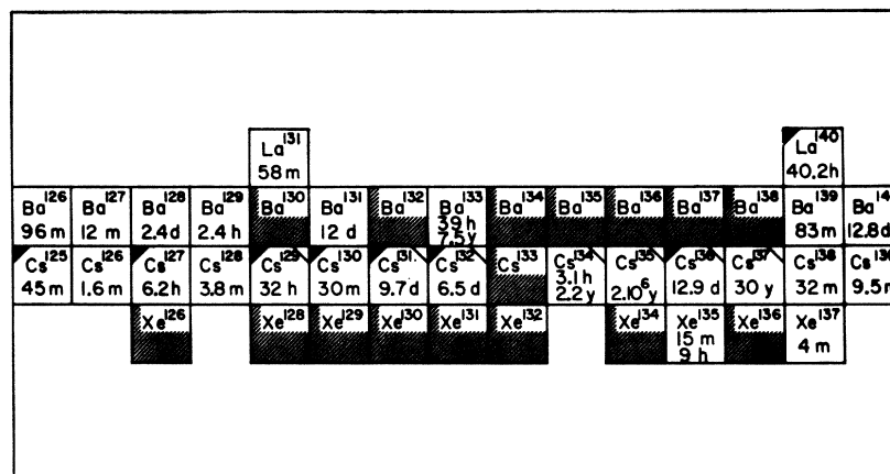
FIG. 1. Nuclides in the cesium region. The nuclides determined mass spectrometrically are indicated by an open triangle in the upper right-hand corner, those measured radiochemically by a filled triangle in the upper left-hand corner. Shaded squares indicate stable nuclides.
