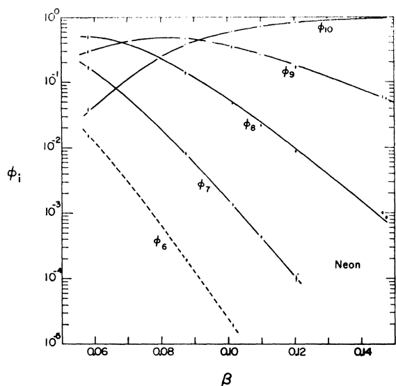
FIG. 6. Equilibrium charge-state distributions for neon as a function of velocity. The dashed curve is not calculated, but serves to connect the experimental points for \phi_6 .
