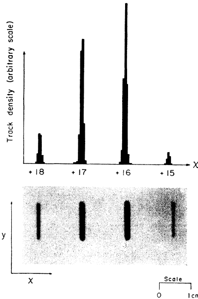
FIG. 2. Film strip in which magnetically separated charge groups Ar +18 through Ar +15 are evident. The measured profile distributions are shown above the film strip. \beta=0.146 ; 50 \mu\text{g}/\text{cm}^2 Zapon foil.
