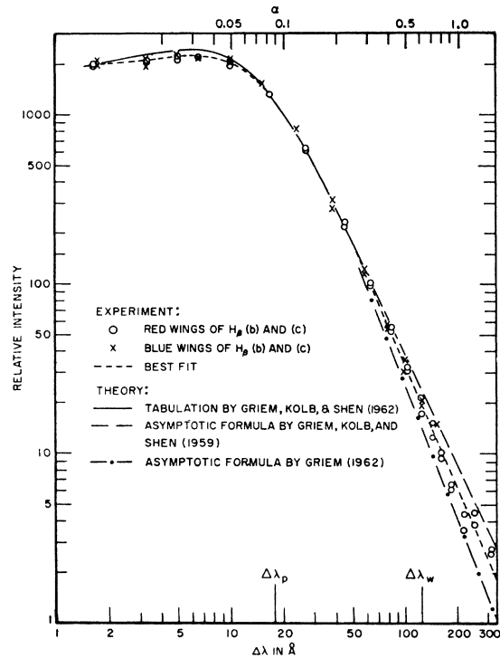
FIG. 6. Comparison of the measured and calculated intensity distribution for H_\beta in logarithmic representation. \Delta\lambda is the distance from the line center. The experimental conditions are the same as in Fig. 3.
