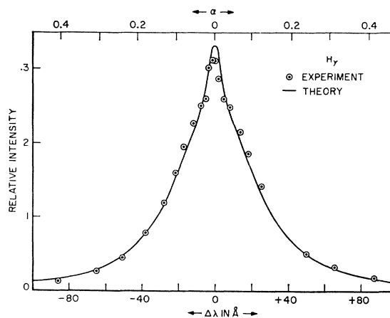
FIG. 4. Comparison of the measured and calculated line profiles for H_\gamma ( N_e = 7.08 \times 10^{16} \text{ cm}^{-3} , T = 12\,460 \text{ K} ).
