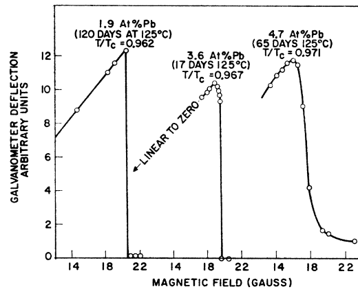
FIG. 4. The variation of Q with magnetic field for three different In-Pb alloys.
