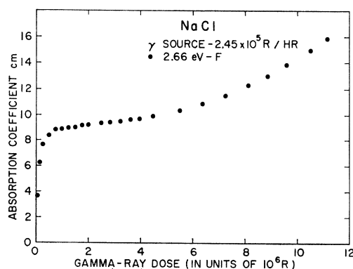
FIG. 1. The absorption coefficient at the peak of the NaCl F -center absorption band vs gamma-ray dose. Usually these curves are referred to as growth or coloring curves.
