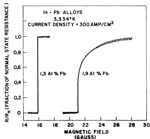
Fig. 2. Resistance transitions for two In-Pb alloys. The transitions broaden in the interval between 1.3 and 1.9 at. % Pb.
