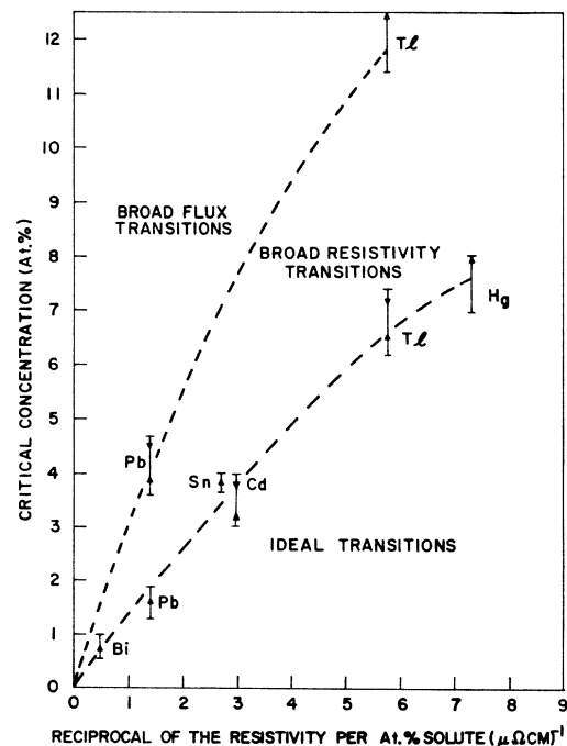
FIG. 8. Critical concentrations of In alloys for ideal superconducting transitions as a function of the reciprocal of the resistivity per at. % solute. The transitions measured by flux and resistive techniques are shown. The extremes indicate the alloys studied on either side of the critical concentration; the arrows indicate which alloy the critical concentration is nearest.
