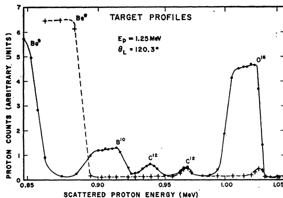
FIG. 5. Profiles of a beryllium target and a target of B 2 O 3 enriched to 94% B 10 , evaporated onto beryllium. The two C 12 peaks on the B 2 O 3 target are attributed to pump oil on the front surface of the B 2 O 3 and on the beryllium surface behind the B 2 O 3 .
