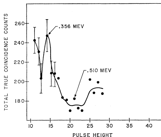
FIG. 5. Gamma-ray spectrum in coincidence with the 0.514-MeV gamma ray of Sr 85 (detectors 90° apart).
