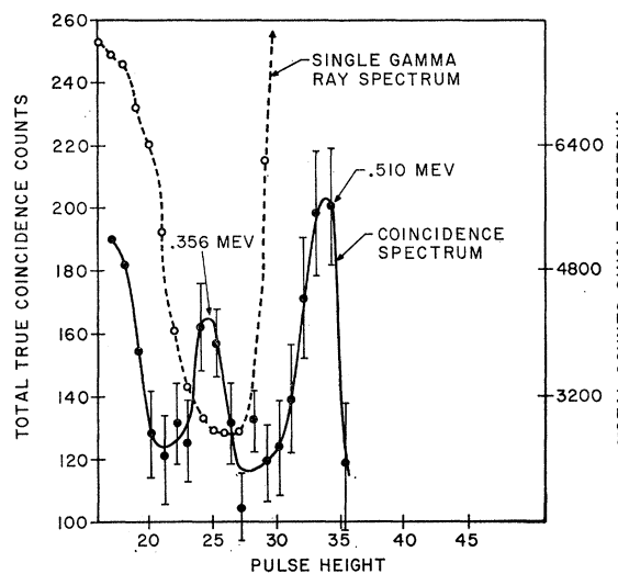
FIG. 4. Gamma-ray spectrum in coincidence with the 0.514-MeV gamma ray of Sr 85 (detectors 180° apart).
