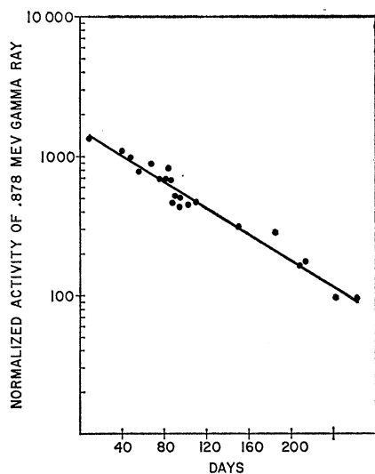
FIG. 1. Half-life measurement of the 0.878-MeV gamma-ray activity of Sr 85 .
