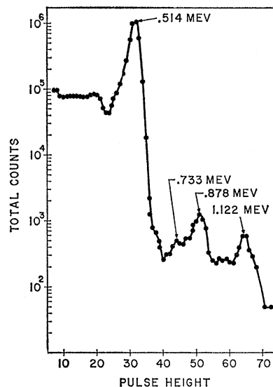
FIG. 2. Gamma-ray spectrum of Sr 85 taken in the course of half-life measurements (2.8 cm of lead inserted between the source and the detector).
