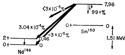
FIG. 2. Proposed partial decay scheme of the s -wave neutron-capturing state of \text{Sm}^{150} .
