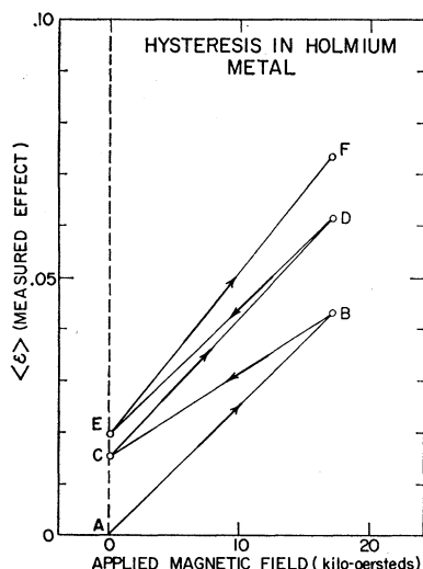
FIG. 4. Hysteresis effects in holmium metal at 0.1°K. The sample, initially in zero applied field at point A, had not been previously magnetized since being cooled down through the Curie point. The magnetic field was first turned on in going from A to B. The field remained at B for 1.5 h while \langle \mathcal{E} \rangle was measured. The field was then turned off in going from B to C. The residual effect which is observed at C is due to retentivity. The cycle was repeated from C to D, D to E, and E to F, always turning the field on in the same direction. As is seen from the figure, two cycles are insufficient to reach saturation.
