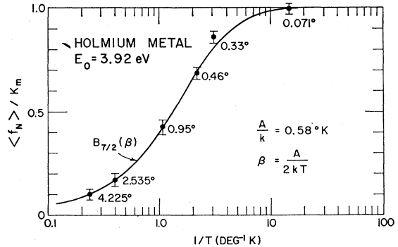
FIG. 3. Observed polarization of holmium nuclei as a function of temperature. The nuclear polarization \langle f_N \rangle was derived from the experimental data using Fig. 2. The value K_m = 0.48 , and the curve (Brillouin function) which is shown are the best fit of the data to Eq. (8). The argument of the Brillouin function corresponds to a hyperfine interaction constant of A/k = 0.58^\circ\text{K} .
