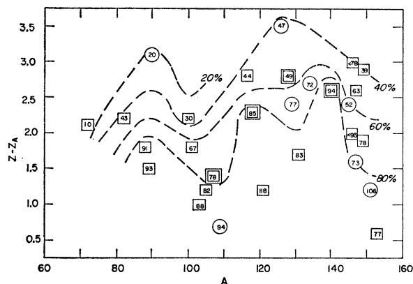
FIG. 8(a). Contour plot of \sigma_c(A,Z)/\sigma_A in the coordinate system Z-Z_A versus A (see text). In Fig. 8(a) and 8(b) the values plotted in double-boxes pertain to data having an accuracy classification of "A" in Table I, those in single boxes pertain to "B," and those in circles pertain to "C."
