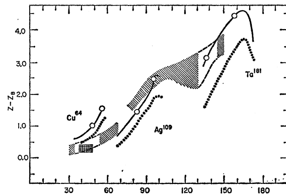
FIG. 12. Comparison of Z_p with the calculated locus of the mean evaporation products for \text{Cu}^{64} excited to energies from 100–500 Mev, and \text{Ag}^{109} and \text{Ta}^{181} excited to energies from 100 to 700 Mev, for a = 0.1 A \text{ Mev}^{-1} (solid lines) and a = 0.05 A \text{ Mev}^{-1} (dotted lines). (See text.)
