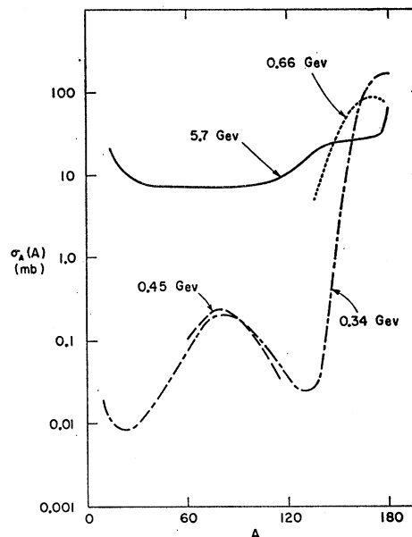
FIG. 7. Comparison of mass yield curves for the interactions of tantalum with high-energy protons. The curve at 0.34 GeV is from Nervik and Seaborg, 22 that at 0.45 GeV is from Kruger and Sugarman, 20 and that at 0.66 GeV is from A. K. Labrukhin and A. A. Pozdnyakov, Sov. J. Atomic Energy 7, 862 (1961).
