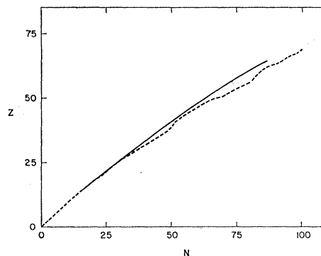
FIG. 9. Comparison of the experimentally-determined locus of isobaric independent yield maxima Z_p (solid line) with the beta-stability line (dashed line).
