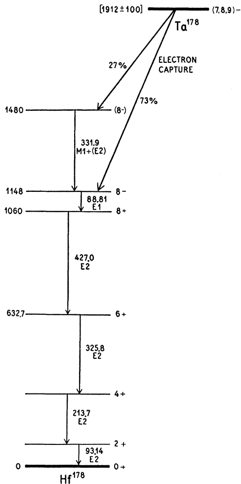
FIG. 1. Decay scheme of 2.1-hr Ta^{178} as reported by Felber, Stephens, and Asaro, 3 and as modified as a result of the measurements of Deutsch and Bauer, 7 Harmatz, Handley, and Mihelich, 5 and the present work.
