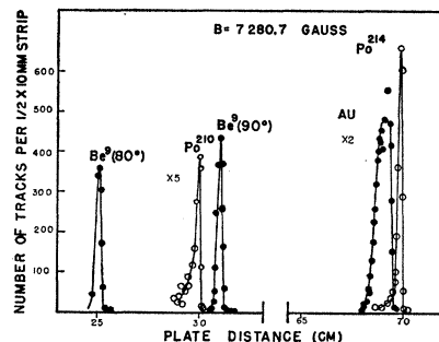
FIG. 1. Particle groups used in comparing the energies of alpha-particles from Po^{214} and Po^{210} . All groups recorded on one plate with a constant magnetic field. The open circles represent alpha-particles and the solid circles represent deuterons. The alpha groups are labelled with the symbol of source. The deuteron groups are labelled with the symbol of the scattering nucleus. Note the break in the abscissa scale.
