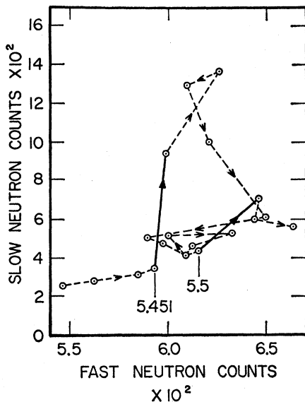
FIG. 5. Slow vs fast neutron counter yields for the 5.451- and 5.5-Mev peaks in Fe^{56}(p, n)Co^{56} . The slow-neutron counter yield is plotted against the fast-neutron counter yield. Successive points in the excitation curve are connected with a dashed line and arrows indicate the direction of increasing energy. Points determining the steepest rise of peaks in the excitation curve are connected with solid lines. As pointed out by Bromley (see reference 6), the slope of the solid line will be nearly vertical when the compound nucleus resonance width overlaps the threshold energy and will fall off as the resonance energy increases above the threshold energy. The slope at 5.451 Mev is much steeper than that observed at 5.5 Mev; consequently, the peak at 5.5 Mev is attributed to a compound nucleus resonance.
