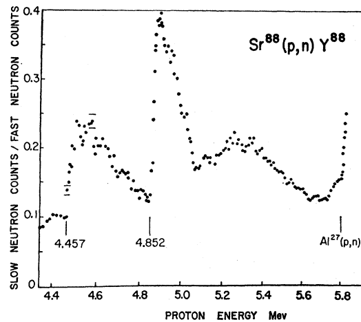
FIG. 4. Counter ratio excitation curve for Sr^{88}(p,n)Y^{88} . Steep rises in the excitation curve at 4.457 and 4.852 Mev were interpreted as ground-state and first-excited state thresholds, respectively.
