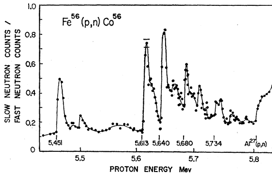
FIG. 3. Counter ratio excitation curve for Fe^{56}(p,n)Co^{56} . The slow- to fast-neutron counter ratio dependence on bombarding energy is plotted up to the Al(p,n) threshold. Thresholds for the ground state and two excited states are indicated by steep rises in the curve. The peak at 5.7 Mev may be due to either a new threshold or resonances in the compound nucleus.
