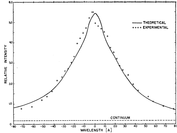
FIG. 6. Comparison of measured and calculated Stark profiles of H_{\gamma} . N_e = 0.94 \times 10^{17} \text{ cm}^{-3} , T = 14\,000 \text{ K} .
