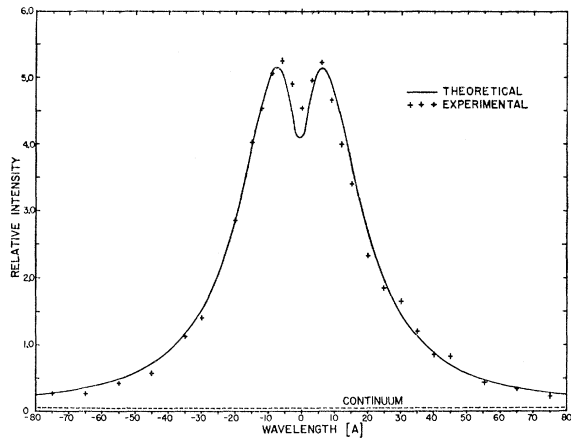
FIG. 5. Comparison of measured and calculated Stark profiles of H_{\beta} . N_e = 0.80 \times 10^{17} \text{ cm}^{-3} , T = 14\,000 \text{ K} .
