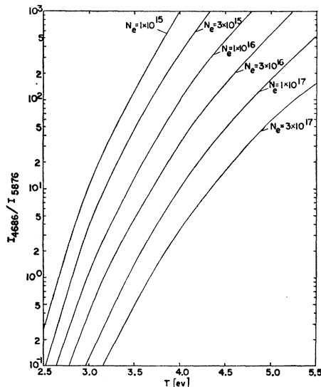
FIG. 2. Intensity ratios of HeII 4686A and HeI 5876A as functions of temperature for various electron densities.
