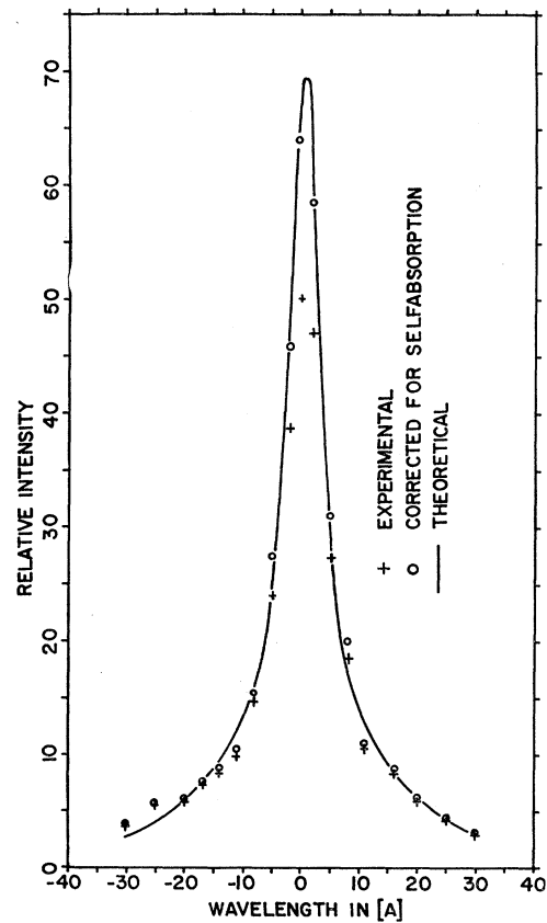
FIG. 4. Comparison of measured and calculated Stark profiles of H \alpha . N_e = 0.92 \times 10^{17} cm ^{-3} , T = 25\,000^\circ\text{K} .
