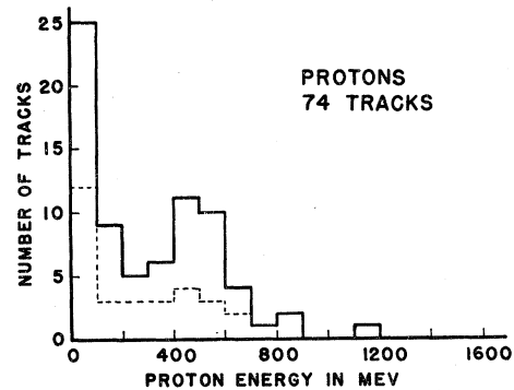
FIG. 3. Center-of-mass system energy distribution of the protons from inelastic events. The solid line is for all protons and the dashed line is for protons from 2-prong events.
