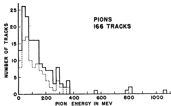
FIG. 4. Center-of-mass system energy distribution of the pions from inelastic events. The solid line is for all pions and the dashed line is for pions from 4-prong events.
