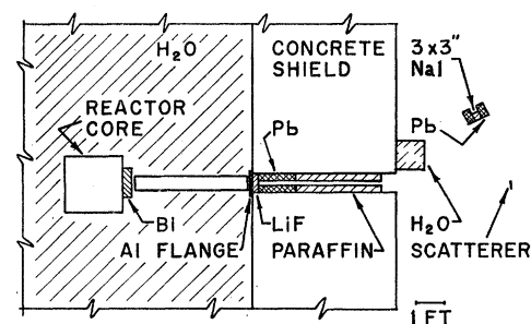
FIG. 1. Experimental arrangement.
