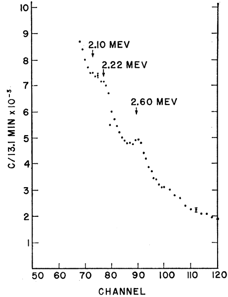
FIG. 3. Signal and background from a \frac{1}{8} -in.-thick scatterer. The 2.22-Mev \gamma rays are from the H^1(n,\gamma)H^2 reaction.
