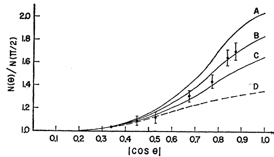
FIG. 6. Relative yield of 2.6-Mev \gamma rays as a function of |\cos\theta| , where \theta is the angle between the incident neutron direction and outgoing \gamma -ray direction. Curves A, B, and C were calculated assuming that the 2.6-Mev state in \text{Pb}^{208} is a 3^- state, and using incident neutron energies of 3.5, 4.1, and 6.0 Mev, respectively. Curve D was calculated assuming the 2.6-Mev state is a 2^+ state, and using an incident neutron energy of 4.1 Mev.
