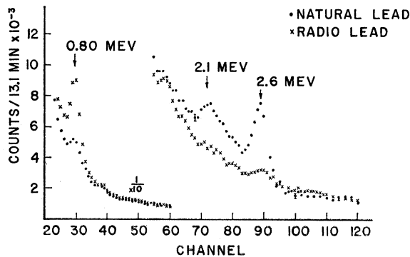
FIG. 2. Gamma rays from Pb(n,n'\gamma)Pb reaction. The dots result from a natural lead target, and the crosses from a radio-lead target. Target thickness was \frac{1}{8} -in.
