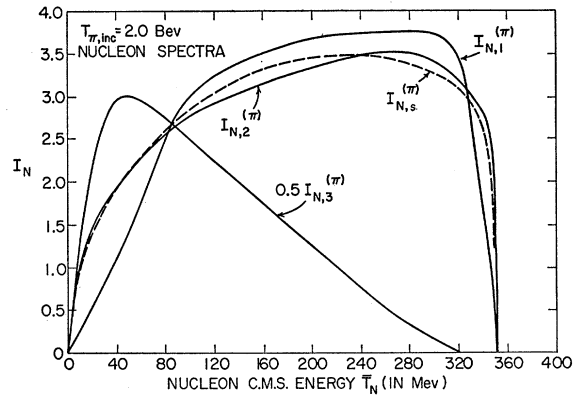
FIG. 9. Center-of-mass energy spectra of nucleons from pion-nucleon interactions at an incident pion energy T_{\pi, inc} = 2.0 Bev. The solid curves show the spectra obtained from the present extended isobar model. The dashed curve gives the result of the Fermi statistical theory.
