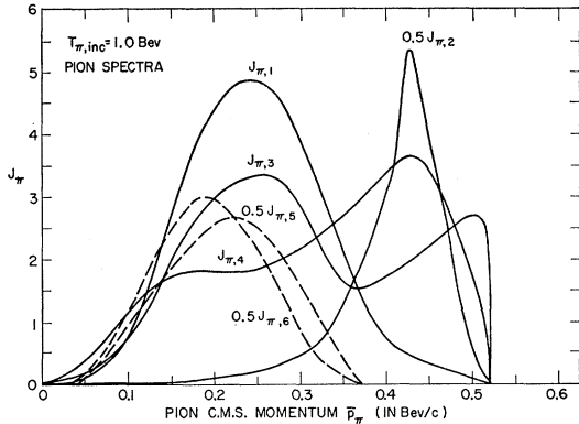
FIG. 2. Center-of-mass momentum spectra of pions from pion-nucleon interactions at an incident pion energy T_{\pi,inc}=1.0 Bev. The spectra J_{\pi,3} and J_{\pi,4} were calculated by including the contribution of the low-energy T=\frac{1}{2} cross section.
