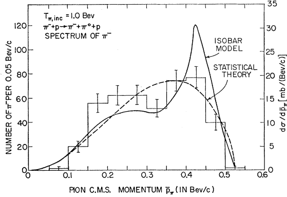
FIG. 12. Center-of-mass momentum spectrum of the \pi^- mesons from the reaction \pi^- + p \rightarrow \pi^- + \pi^0 + p at T_{\pi, \text{inc}} = 1.0 Bev. The histogram represents the combined experimental data from references 24–26. The solid curve was obtained from the present extended isobar model. The dashed curve gives the result of the Fermi statistical theory.
