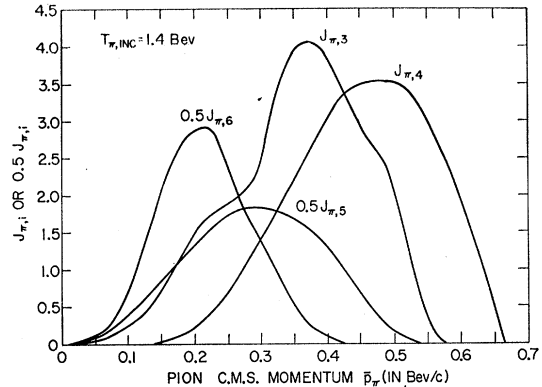
FIG. 6. Center-of-mass momentum spectra of pions from pion-nucleon interactions at an incident pion energy T_{\pi,inc} = 1.4 BeV. The spectra J_{\pi,3} and J_{\pi,4} were obtained by neglecting the low-energy T = \frac{1}{2} cross section.
