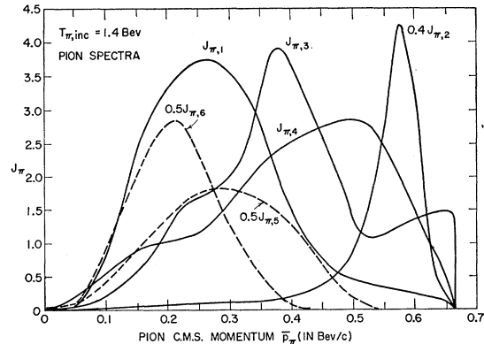
FIG. 3. Center-of-mass momentum spectra of pions from pion-nucleon interactions at an incident pion energy T_{\pi,inc}=1.4 Bev. The spectra J_{\pi,3} and J_{\pi,4} were calculated by including the contribution of the low-energy T=\frac{1}{2} cross section.
