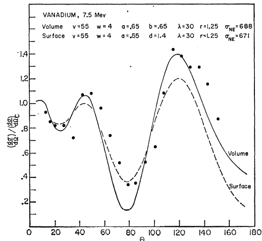
FIG. 2. Elastic scattering from vanadium. Curves show typical best fits for VA- and SA-type potentials to experiments (notation and units same as Fig. 1).
