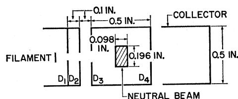
FIG. 2. Diagram of low-energy electron gun. The ac attenuation of the electron beam is measured at the collector. The electron beam holes D_1 , D_2 , D_3 , and D_4 are 0.08, 0.08, 0.100, and 0.120 in. in diameter, respectively.
