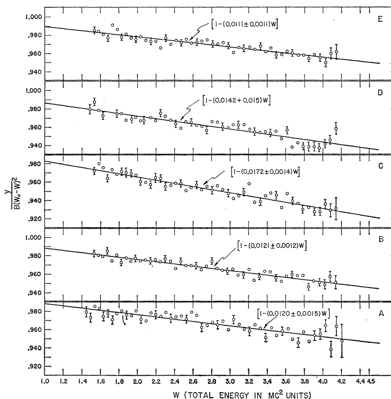
FIG. 7. \text{P}^{32} shape-factor plots.
