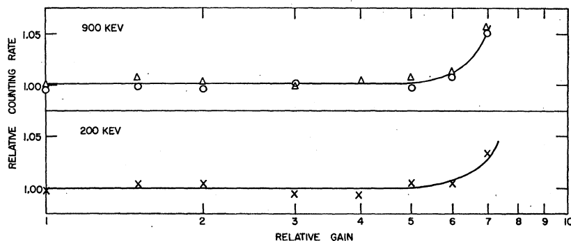
FIG. 2. Scintillation detection plateaus for two electron energies.
