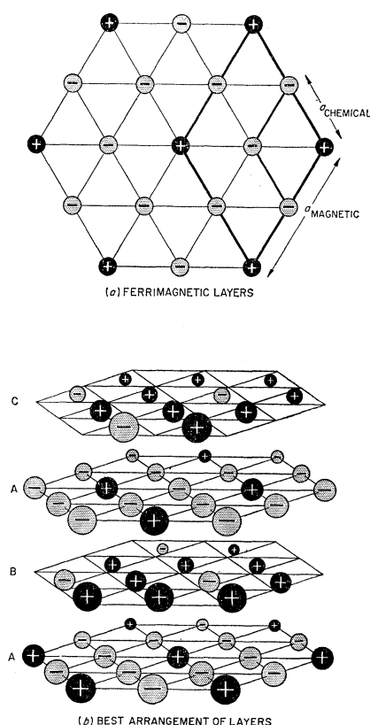
FIG. 4. Possible antiferromagnetic ordering in the hcp phase of cerium.
