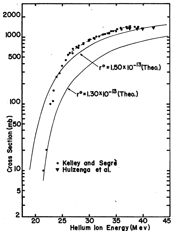
FIG. 14. Total cross-section data for the (\alpha, xn) reaction on bismuth (Kelly and Segrè 13 and Hulzenga et al. 10 ) for various helium ion energies.
