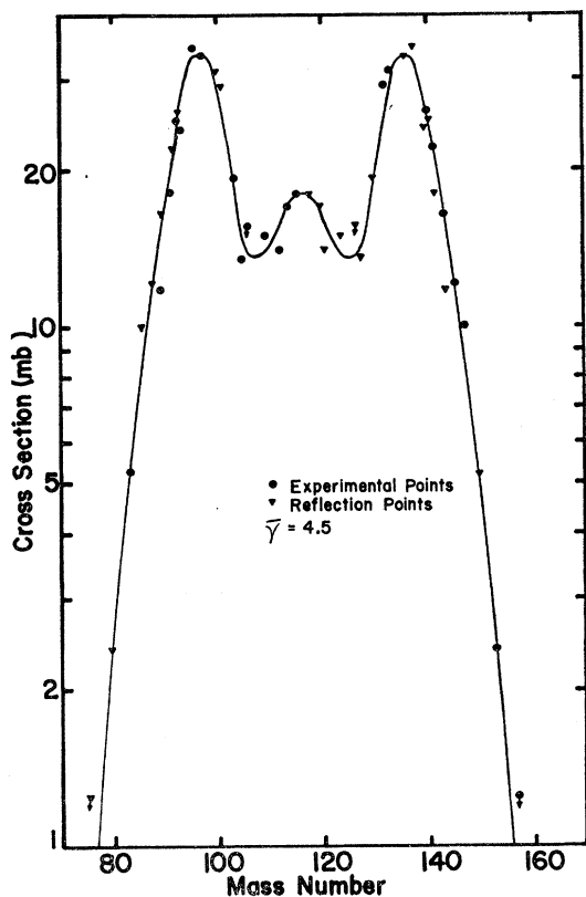
FIG. 3. Fission mass yield curve for 29.0-Mev helium ions on U^{238} .
