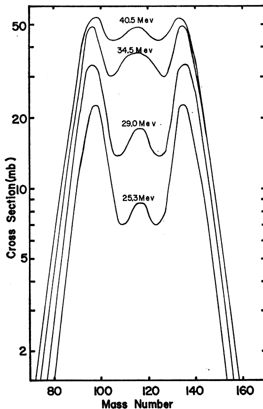
FIG. 11. Composite fission mass yield curves for medium-energy helium ions on U^{238} .
