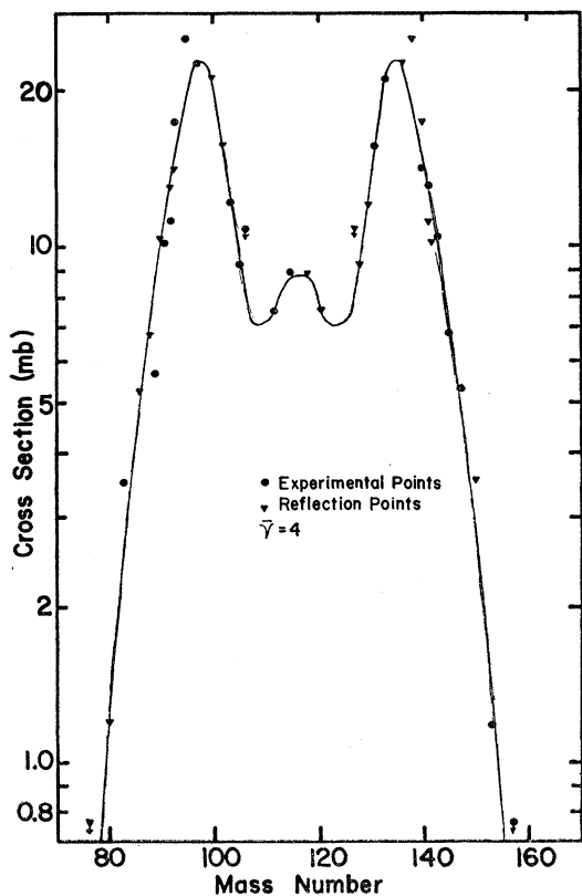
FIG. 4. Fission mass yield curve for 25.3-Mev helium ions on U^{238} .
