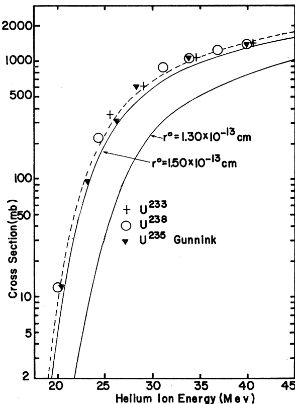
FIG. 13. Total reaction cross sections for U^{233} , U^{235,16} and U^{238} at various helium ion energies and a comparison with compound nucleus theory assuming the square-well potential (Blatt and Weisskopf 2 ).
