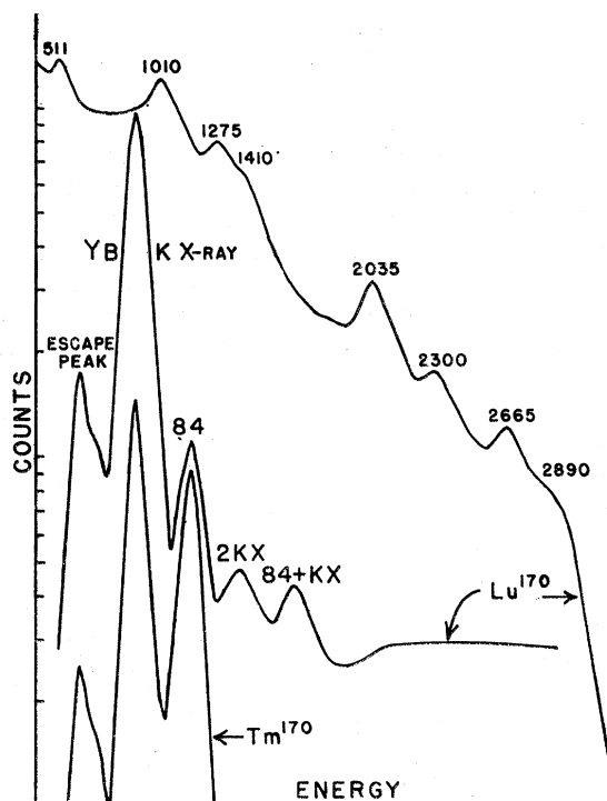
FIG. 1. Gamma-ray spectrum of Lu 170 as measured with a 3×3 inch crystal and a 100-channel scintillation spectrometer. Sample was centered on flat face of crystal.
