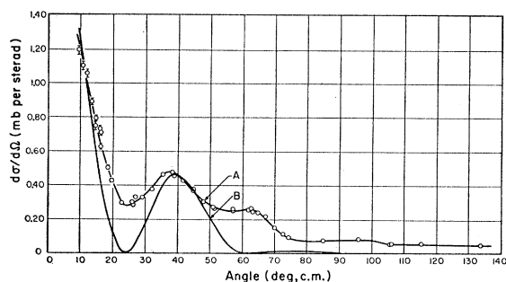
FIG. 7. Angular distribution of deuterons from formation of the ground state of N^{14} . Curve A presents the experimental results; Curve B, calculated results from the El Nadi equation using l_n=l_p=1 , r=4.57 fermis.
