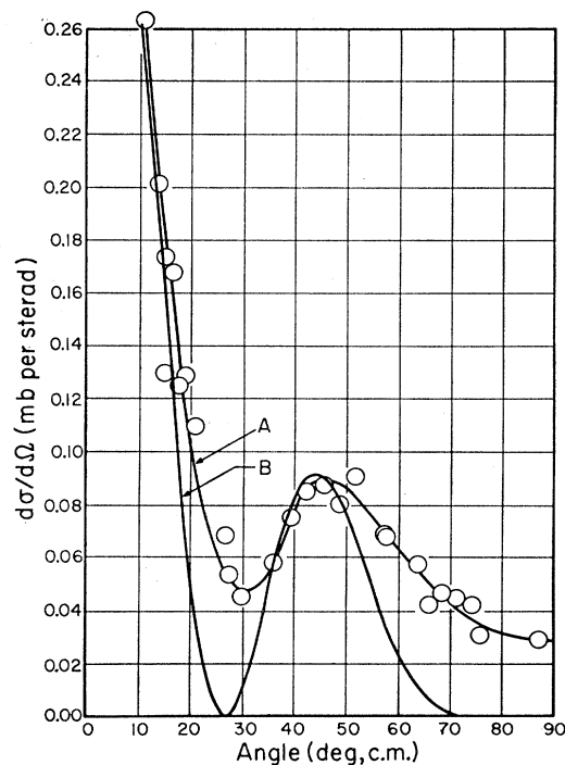
FIG. 8. Angular distribution of deuterons from formation of the 3.95-Mev level of N^{14} . Curve A presents the experimental results; Curve B, calculated results from the El Nadi equation using l_n=l_p=1 , r=4.22 fermis.
