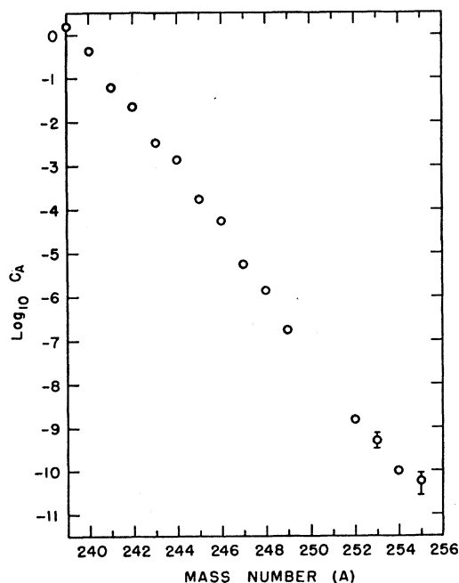
FIG. 3. The \log_{10} of the cumulative abundances ( C_A ) at the time of the detonation of Mike. C_A = N_A + N_{A+1} + N_{A+2} + \dots + N_{255} .
