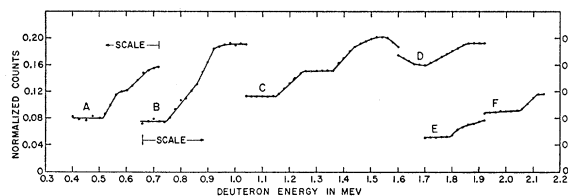
FIG. 2. The "normalized" high-energy gamma-ray counts as a function of bombarding energy. For the different regions of the curve, the following information is given: the ordinate scale (left or right) and the energy windows used to obtain the ordinate value (the numerator and denominator). A—left scale, 8.7-10.0 and 6.4-11.4 Mev. B—right scale, 9.5-11.5 and 6.3-11.5 Mev. C—right scale, 10.0-11.3 and 7.3-12.5 Mev. D—right scale, 10.5-11.8 and 7.8-13.0 Mev. E—right scale if numbers are multiplied by five, 9.8-10.8 and 7.8-13.0 Mev. F—right scale, 12.0-13.0 and 9.0-13.2 Mev. The reasons for these energy windows and the method of analysis are discussed in the text. The existence of thresholds at 0.60 and 0.85 Mev is not certain.
