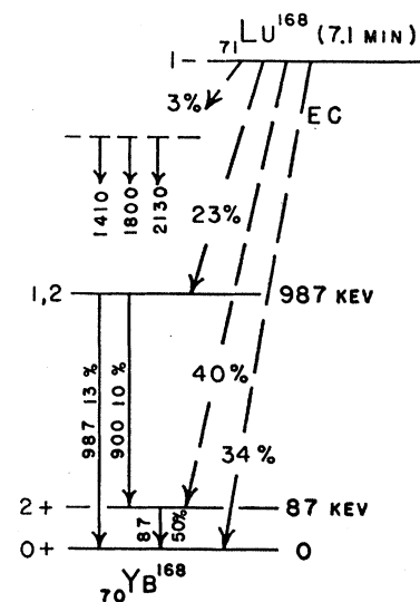
FIG. 1. Proposed energy level scheme for the decay of \text{Lu}^{168} .
