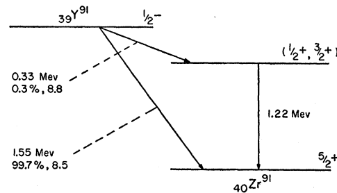
FIG. 1. The decay scheme of Y 91 as proposed by Way et al., see reference 2, based on compiled nuclear data.
