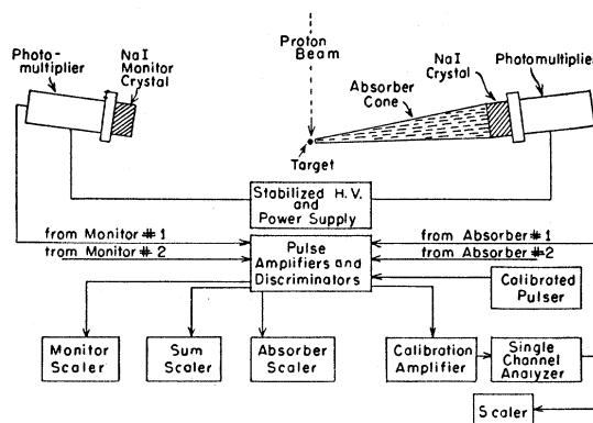
FIG. 1. Schematic experimental arrangement.
