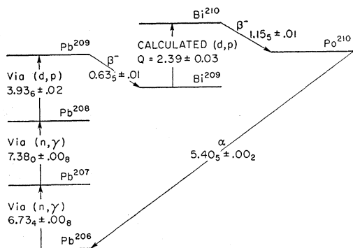
FIG. 1. The closed mass-cycle illustrating the expected Q for the Bi^{209}(d,p)Bi^{210} reaction (references 8 and 12). A new group found in the present investigation has a measured Q = 2.35 \pm 0.03 Mev, in agreement with the expected ground-state value of 2.39 \pm 0.03 Mev. The error quoted for the expected value is the rms error of all of the contributing measurements shown.
