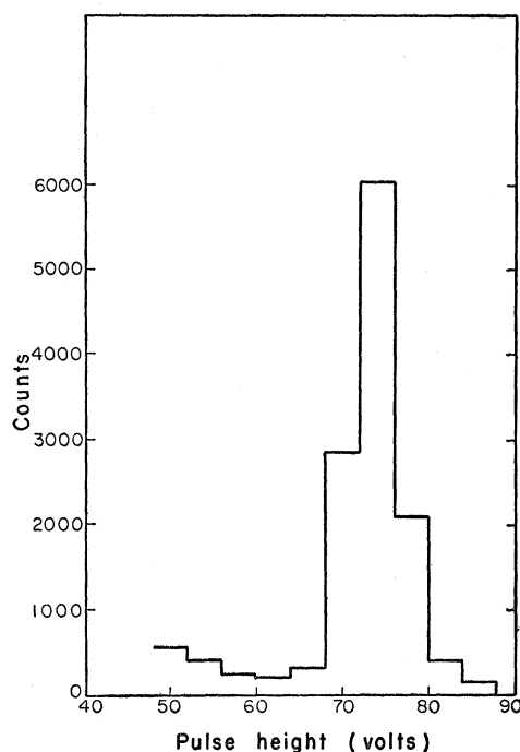
FIG. 1. Pulse-height spectrum of alpha particles scattered from helium at E_{\text{lab}} = 41.9 Mev; \theta_{\text{lab}} = 32.5^\circ .
