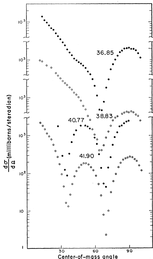
FIG. 2. Differential cross sections for elastic alpha-alpha scattering at laboratory energies from 36.85 to 41.90 Mev.
