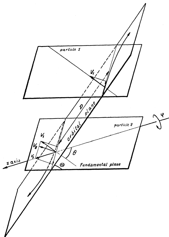
Fig. 1. Space diagram for encounter between charged particles. The fundamental plane is defined by the vectors \mathbf{v}_1 and \mathbf{v}_2 representing the velocities of the two particles before the encounter. The velocity of the mass center denoted by V_c , remains constant during the encounter. In a frame of reference in which the center of gravity is at rest, the two particles describe hyperbolas or parabolas in the orbital plane which, in general, is inclined at some definite angle \Theta to the fundamental plane.
