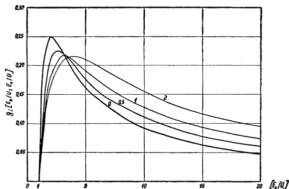
FIG. 4. Plot of the function g_j .
