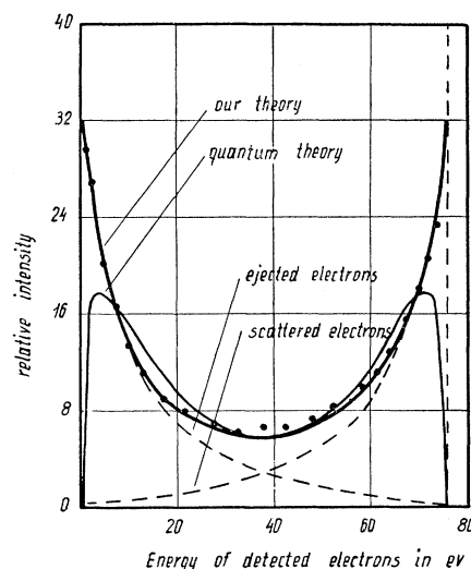
FIG. 5. Velocity distribution of ejected and scattered electrons resulting from ionizing collisions with helium atoms.
