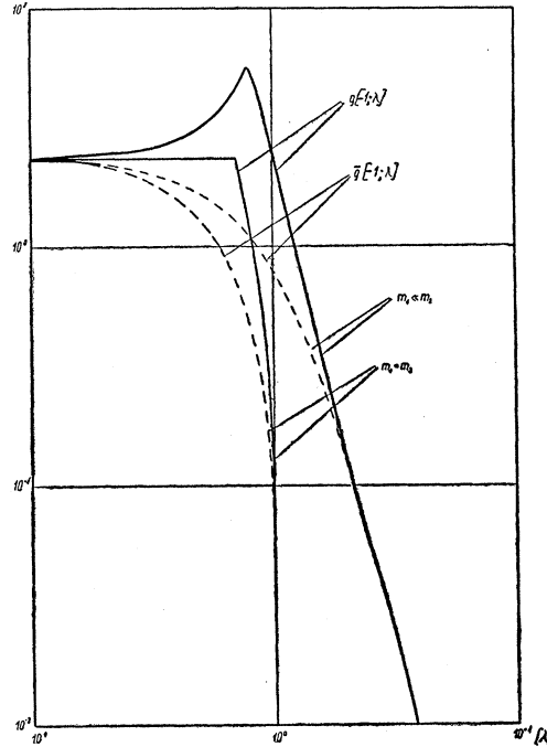
FIG. 3. Values of functions g[\Delta, \lambda] and \bar{g}[\Delta, \lambda] for \Delta E = -E_1 , m_1 = m_2 , and m_1 < m_2 versus the ratio v_2/v_1 .
