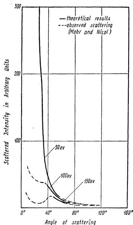
FIG. 12. The angular distribution of inelastically scattered electrons from H_2 for various loss of energy (50,000, and 150 eV).
