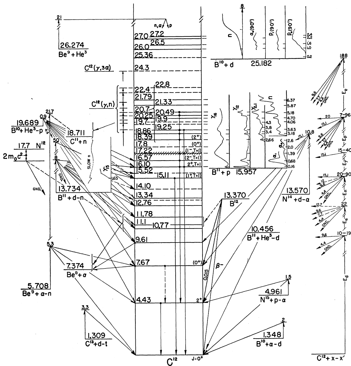
FIG. 1. Energy level diagram of C^{12} , after Ajzenberg and Lauritsen (reference 1) with some additions.
