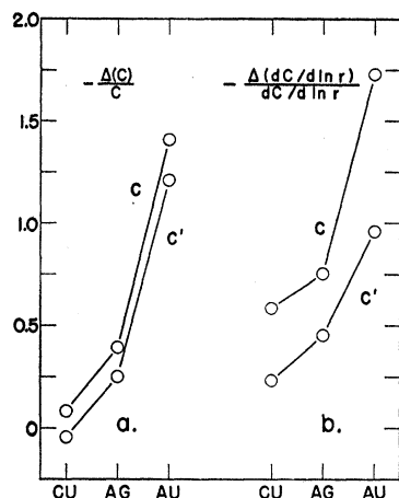
FIG. 2. Closure failures \Delta expressed as fractions of the corresponding total experimental quantity. (a) Elastic shear constants; (b) hydrostatic strain derivatives of shear constants.
