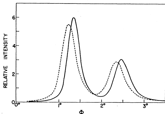
FIG. 6. Before and after irradiation. The diffractometer profile of the (400) Co K\alpha doublet near 10°K. Initial profile (solid line); final profile (dashed line). Here \Phi = \theta - \theta_0 , where \theta is the Bragg angle (about 83°) and \theta_0 is an arbitrary reference angle. The profile shows 18% broadening due to macroscopic bending of the specimen crystal. The bending agrees with that predicted by displacement-theory calculations of inhomogeneity of damage through the thickness of the crystal.
