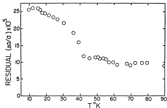
FIG. 4. Thermal recovery of irradiation-induced lattice expansion.
