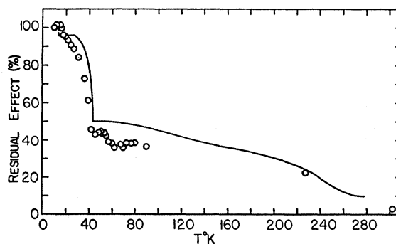
FIG. 7. Thermal recovery of deuteron damage in copper. \circ The present lattice expansion measurements; — electrical resistivity (Cooper et al. , 3 Run II; --- indicates the effect of an initial one-minute temperature pulse to near 30°K).
