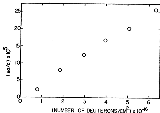
FIG. 3. Crystal lattice expansion under deuteron irradiation near 10°K. Changes in (400) interplanar spacing of single-crystal copper for incident deuteron energy near 7 Mev.
