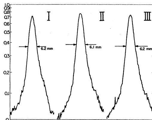
FIG. 5. Diffraction line width on film. Typical microphotometer records of films taken below 10°K before irradiation (I), after irradiation (II), and after irradiation and annealing at 302°K (III). No apparent line broadening is produced by an irradiation of 6.3 \times 10^{16} deuterons/cm 2 .
