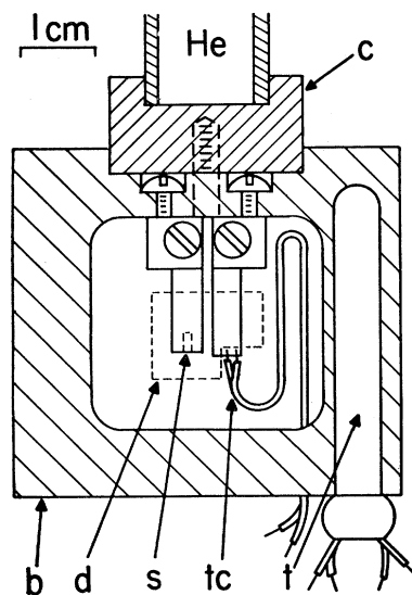
FIG. 2. Vertical section of specimen block assembly. c = tail of cryostat, b = OFHC copper block, d = cross section of deuteron beam, s = region on specimen crystal studied by x-rays, tc = dummy foil thermocouple, t = platinum resistance thermometer. The block has front and back faceplates as thermal radiation shielding for the specimen; the deuteron and x-ray ports subtend only about \pi/3 steradian.
