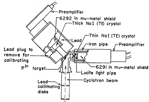
FIG. 3. Arrangement of scintillation detectors used in the coincidence experiments.
