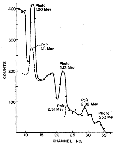
FIG. 6. Energy spectrum of gamma rays in coincidence with the proton group corresponding to the second excited state of S^{34} in the reaction P^{31}(\alpha, \beta)S^{34} . The correction for accidental coincidences has been made.
