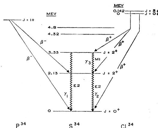
FIG. 7. Excited states of S^{34} .
