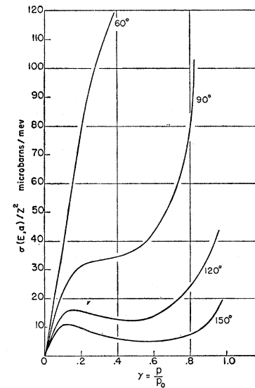
FIG. 1. \sigma(E, \alpha)/Z^2 as a function of \gamma = p/p_0 , \alpha being held fixed at various values. p and p_0 are the outgoing and incident moment of the electron. p_0 = 4mc and \sigma/Z^2 is measured in microbars/Mev.
