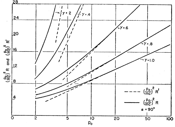
FIG. 2. (p_0/m)^2 R and (p_0/m)^2 R' plotted against \log p_0 , \gamma and \alpha being held fixed at various values. The dotted straight lines correspond to R' , the approximate high-energy large-angle result. \alpha is 90° for each curve. \gamma = p/p_0 , where p and p_0 are the outgoing and incident momenta of the electron.
