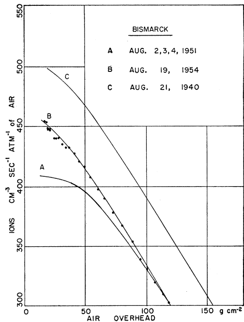
Fig. 11. Comparison of ionization curves of 1954 and 1940. All possible particles were not getting to the earth in 1954, as indicated by curve C taken in 1940.
