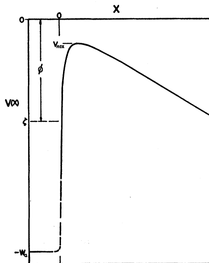
FIG. 1. Potential energy of an electron near the metal surface, Eqs. (3) and (4).
