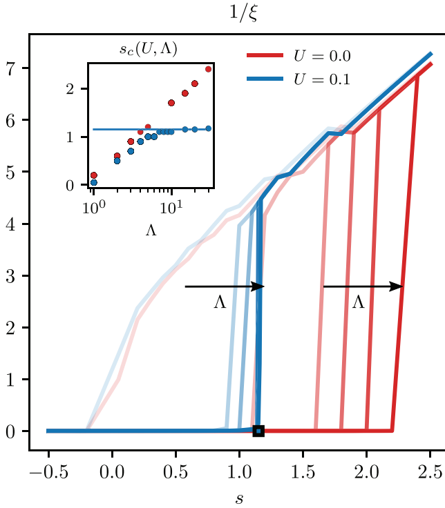
FIG. 4. The inverse of the localization length \xi in a system of L = 15 “active” sites in the symmetry sector n_0 = 1 and \beta_r=0 . The main plot shows the inverse of the localization length \xi^{-1} as a function of s for different values of \Lambda \in [1, 30] and U . The darker lines correspond to larger values of \Lambda . The square is the mean-field estimate of s_c in the bosonic case ( \Lambda = \infty ). The inset shows the behavior of s_c(U, \Lambda) as a function of \Lambda for U = 0 (red) and U = 0.1 (blue). The circles correspond to numerically extracted values from the DMRG results, while the continuous lines are the mean-field estimate s_c \approx \log(1/\sqrt{U}) , which matches the numerics at large \Lambda .
