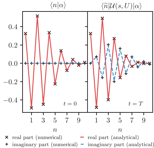
FIG. 7. At t = 0 , the system is prepared in a single-body coherent state |\alpha\rangle = |\alpha\rangle_0 \otimes_{j=1}^L |0\rangle_j , where |\alpha\rangle_0 is a coherent state on the first site with \alpha = 1.5 . At time t \geq 0 , we apply the adiabatic protocol defined in Eq. (11) to the state |\alpha\rangle up to time t = T , obtaining |\tilde{\alpha}'\rangle . In the left panel, we compute the probability amplitudes \langle n|\alpha\rangle , where |n\rangle = |n\rangle_0 \otimes_{j=1}^L |0\rangle_j is an eigenstate of the number operator \hat{n}_0 . The data (symbols) match the amplitudes of a single-site coherent state with \alpha = 1.5 (continuous and dashed line). In the right panel, we compute the probability amplitudes \langle \tilde{n}|\mathcal{U}(s, U)|\alpha\rangle , where |\tilde{n}\rangle is a superboson [cf. Eq. (10)] with n excitations on the first site. The data (symbols) match the amplitudes of the localized version of a coherent state defined in Eq. (17) well, with \alpha' = 1.5e^{1.42i} (continuous and dashed line).
