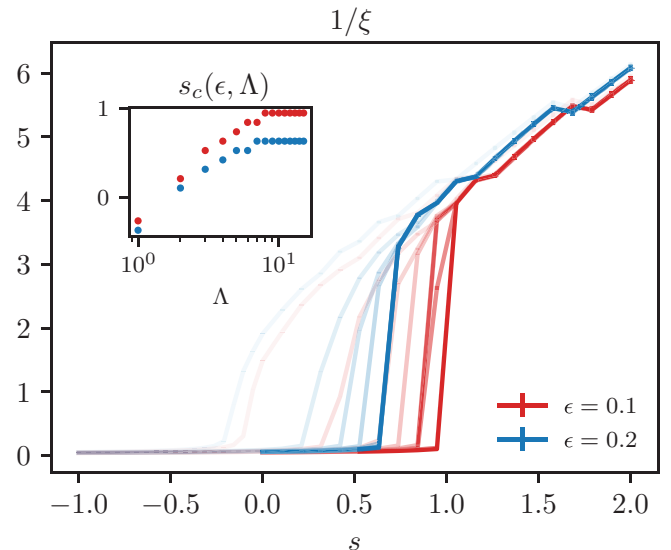
FIG. 12. The inverse of the localization length \xi in a system of L = 15 “active” sites in the symmetry sector n_0 = 1 , \beta_{r=0} . The main plot shows the inverse of the localization length \xi^{-1} as a function of s for different values of \Lambda \in [1, 15] and \epsilon at U = 0 . The darker lines correspond to larger values of \Lambda . The inset shows the behavior of s_c(\epsilon, \Lambda) as a function of \Lambda for \epsilon = 0.1 (red) and \epsilon = 0.2 (blue) at U = 0 .
