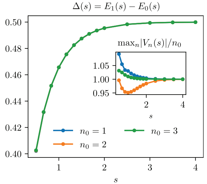
FIG. 6. The gap of the Hamiltonian in Eq. (5) as a function of s \in [0.5, 4] for different values of the occupation n_0 of the first nonempty site. The inset shows the maximum matrix element \max_n |V_n(s)|/n_0 \equiv \max_n \langle \psi_n(s) | V | \psi_0(s) \rangle / n_0 of the perturbation V = \sum_j \hat{n}_j (\hat{a}_{j+1} + \hat{a}_{j+1}^\dagger) between the n th excited state and the ground state at fixed s . We fix a system size L = 6 , cutoff \Lambda = 3 , and nearest-neighbor density-density interaction U = 1 . The transition point is at s_c(U = 1) \approx 0 . The results are weakly affected (of the order of few percent) by the finite cutoff \Lambda for s \lesssim 2 .
