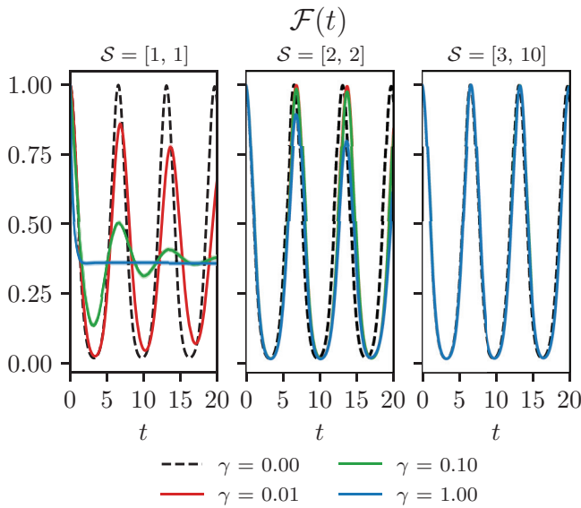
FIG. 11. The dynamics of the fidelity [cf. Eq. (24)] of a supercat state with \alpha = 1.5 upon changing the noise strength \gamma and its support \mathcal{S} = [a, b] , starting from site a and ending at site b . We fix U = 1 and s = 1.5 . The initial state is exponentially localized around the site j = 1 . The dephasing is highly disruptive only in an exponentially localized region around the peak (see the first two columns). Instead, if it acts on a region far from the localized peak, it does not produce any appreciable effect at the scale shown in the plots. The light area surrounding the curves represents the statistical error due to the finite number of sampled trajectories.
