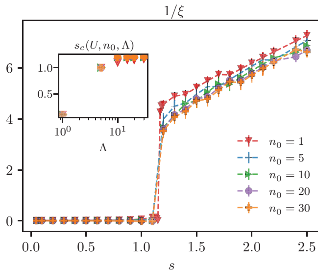
FIG. 13. The inverse of the localization length \xi in a system of L = 15 “active” sites upon changing s for different values of n_0 = 1 . We fix U = 0.1 . The main plot shows the inverse of the localization length \xi^{-1} as a function of s for \Lambda = 30 . The inset shows the behavior of s_c as a function of \Lambda for different values of n_0 . The circles correspond to numerically extracted values from DMRG results. The points are indistinguishable upon changing n_0 for \Lambda \gtrsim 10 .
