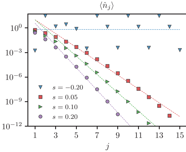
FIG. 2. The average occupation number of the ground state for different values of s at fixed nearest-neighbor density interaction U = 1 . We fix L = 15 , a cutoff \Lambda = 30 to the maximal occupation number, and n_0 = 1 . In the plot, we do not display the occupation n_0 of the zeroth site that fixes the “East symmetry” sector. The dashed lines are the exponential fit, the slope of which is -1/\xi , where \xi is the localization length [cf. Eq. (6)].
