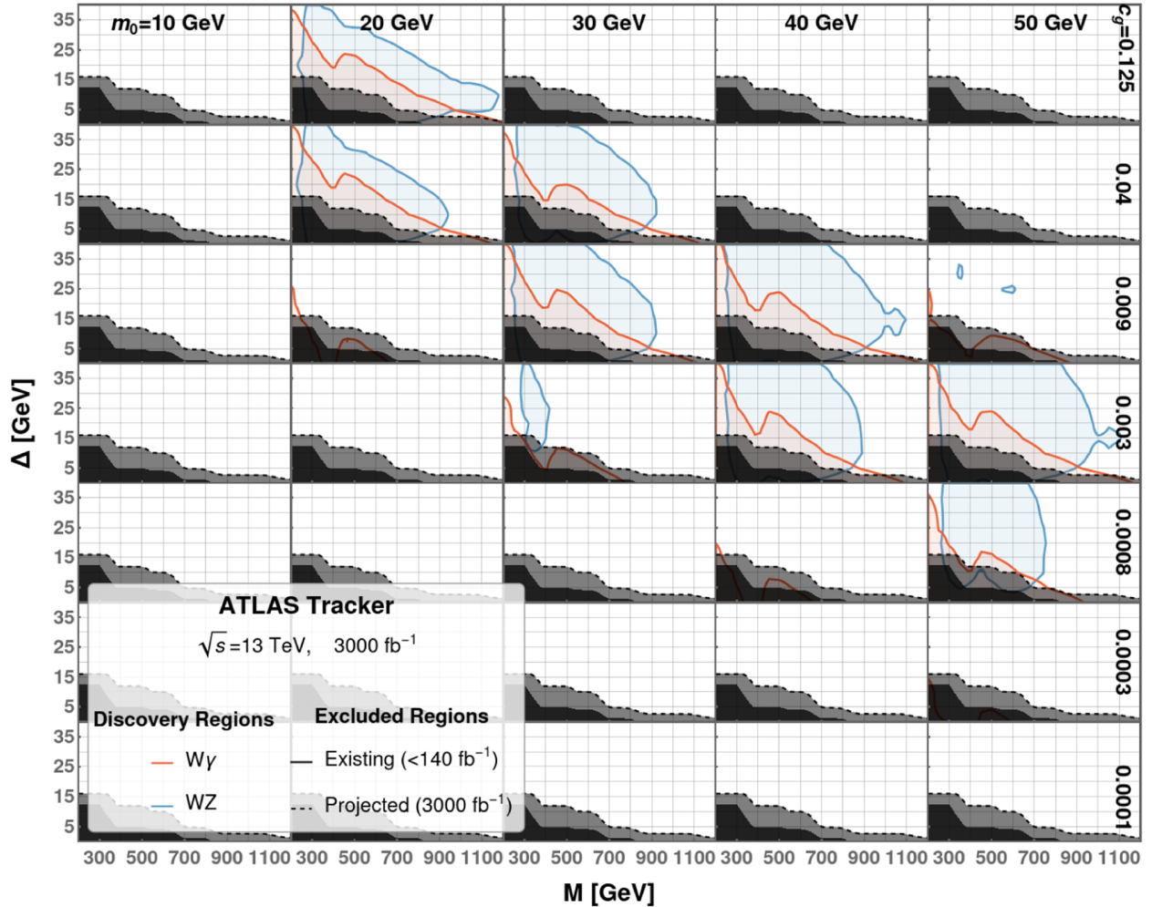
FIG. 8. Exclusion and simulated discovery regions in M and \Delta inside the ATLAS Tracker at \sqrt{s} = 13 TeV and 3000 \text{ fb}^{-1} for various (c_g, m_0) . Exclusion regions in black are due to W\gamma resonance searches by ATLAS [44] and CMS [46]. Simulated discovery regions in orange (blue) indicate five or more events at a given (M, \Delta) with a 0^{++} hidden sector glueball decay within the tracker and a W^\pm\gamma ( W^\pm Z ) decay which passes the appropriate cuts (see Appendix A 6).
