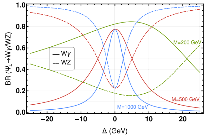
FIG. 4. Branching ratios for a charged bound state \Psi_{\pm} decaying into W\gamma/WZ as a function of the squark mass splitting ( \Delta ) for various total masses ( M ). The W\gamma signal dominates at small \Delta , but quickly turns over at a few GeV. The turnover point decreases in \Delta as M increases.
