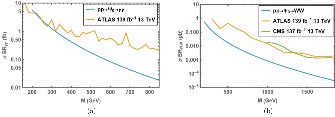
FIG. 3. Potential collider bounds from SM final states of decays of the neutral squark bound state \Psi_0 . On the left (right) the bound is from decays into \gamma\gamma ( WW ), assuming a conservative branching fraction of 1% (100%). We see that there is a lower bound on the combined squark mass M from diphoton searches.
